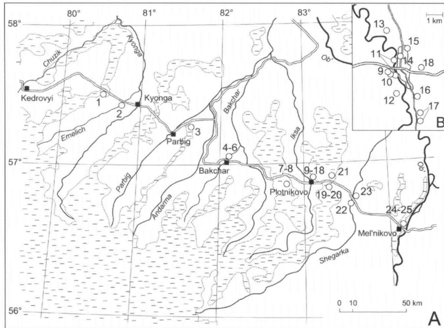
Fig. 1. Situation of studied localities: (A) in the investigated area; – (B) in the environs of Plotnikovo. Numbers correspond to the locality numbers given in the text.
